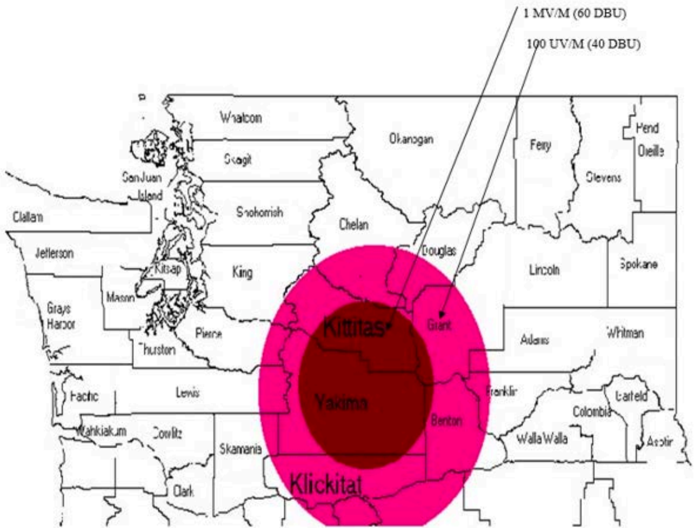
COVERAGE MAP SHOWING PREDICTED CONTOURS OF KDNA (FM) YAKIMA WA
