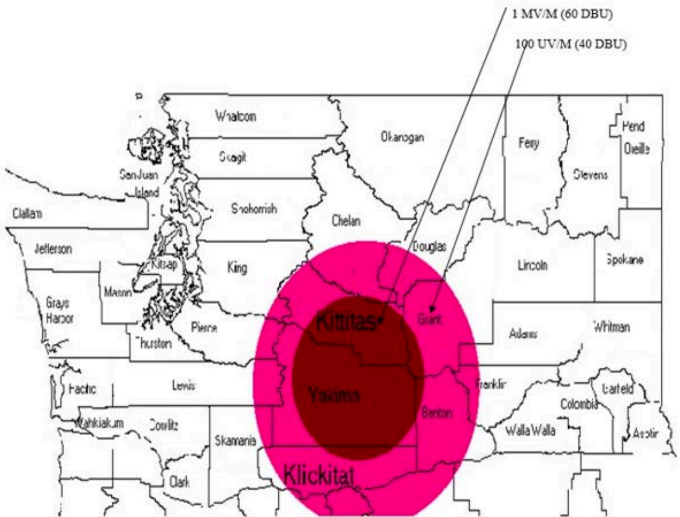
COVERAGE MAP SHOWING PREDICTED CONTOURS OF KDNA (FM) YAKIMA WA
